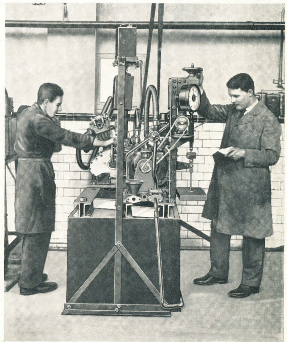
A ROYAL ENFIELD “BULLET” ENGINE BEING TESTED IN THE DYNAMOTOR HOUSE.
