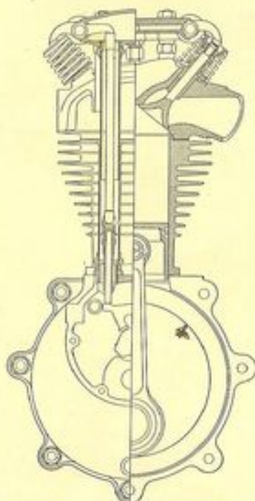
Sectional diagram of new 3.46 h.p. O.H.V. engine.
