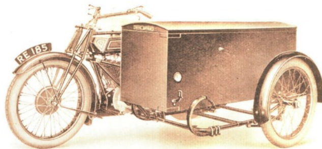
9.76 H.P. TRADE DELIVERY COMBINATION MODEL 185
